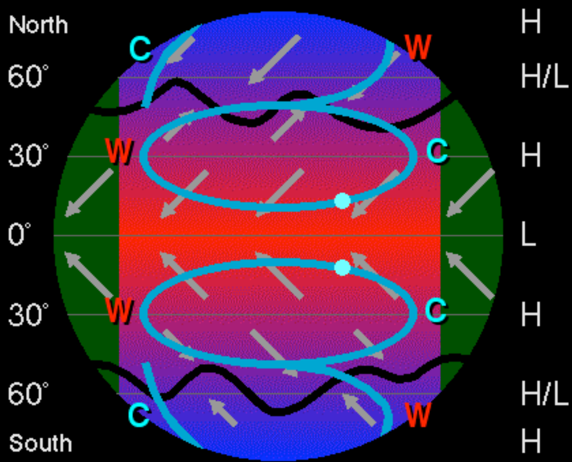
Ocean Surface Circulation
