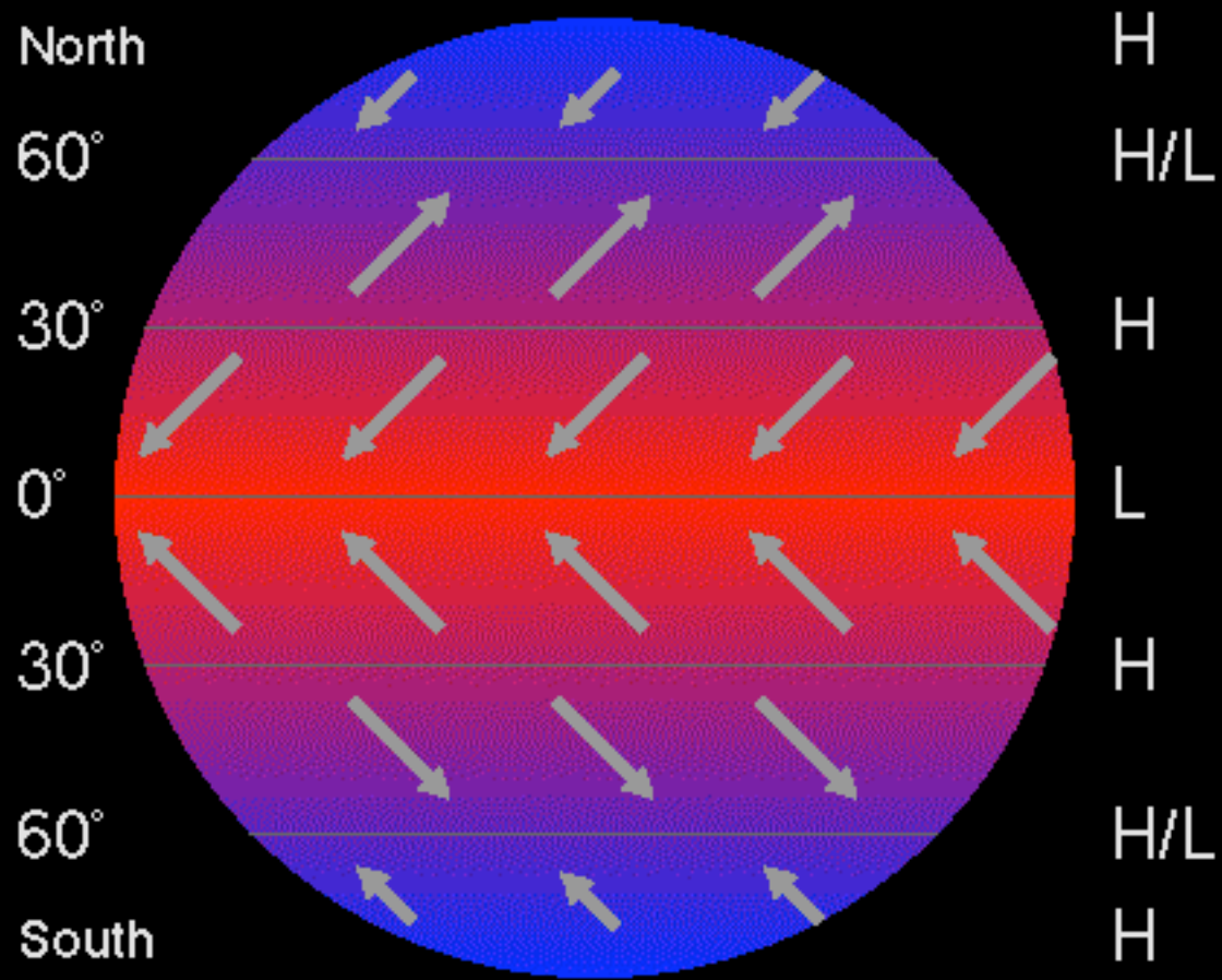
Coriolis Surface Windfield
