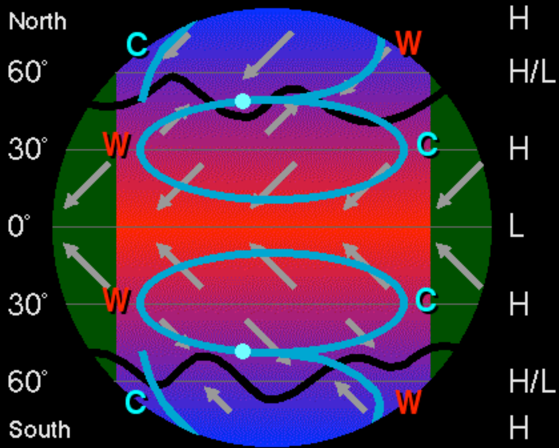
Ocean Surface Circulation
