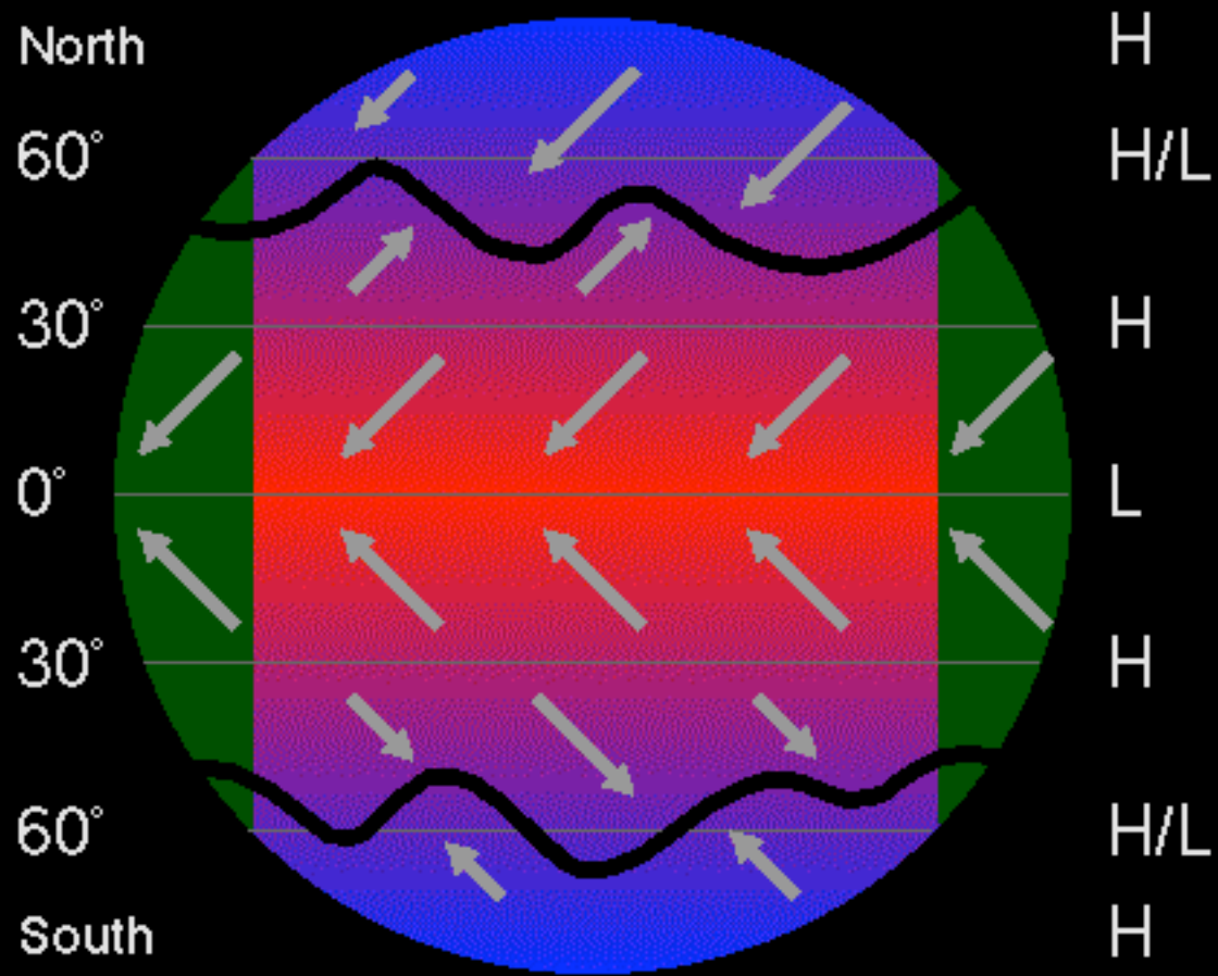
Coriolis Surface Windfield w/Continents
