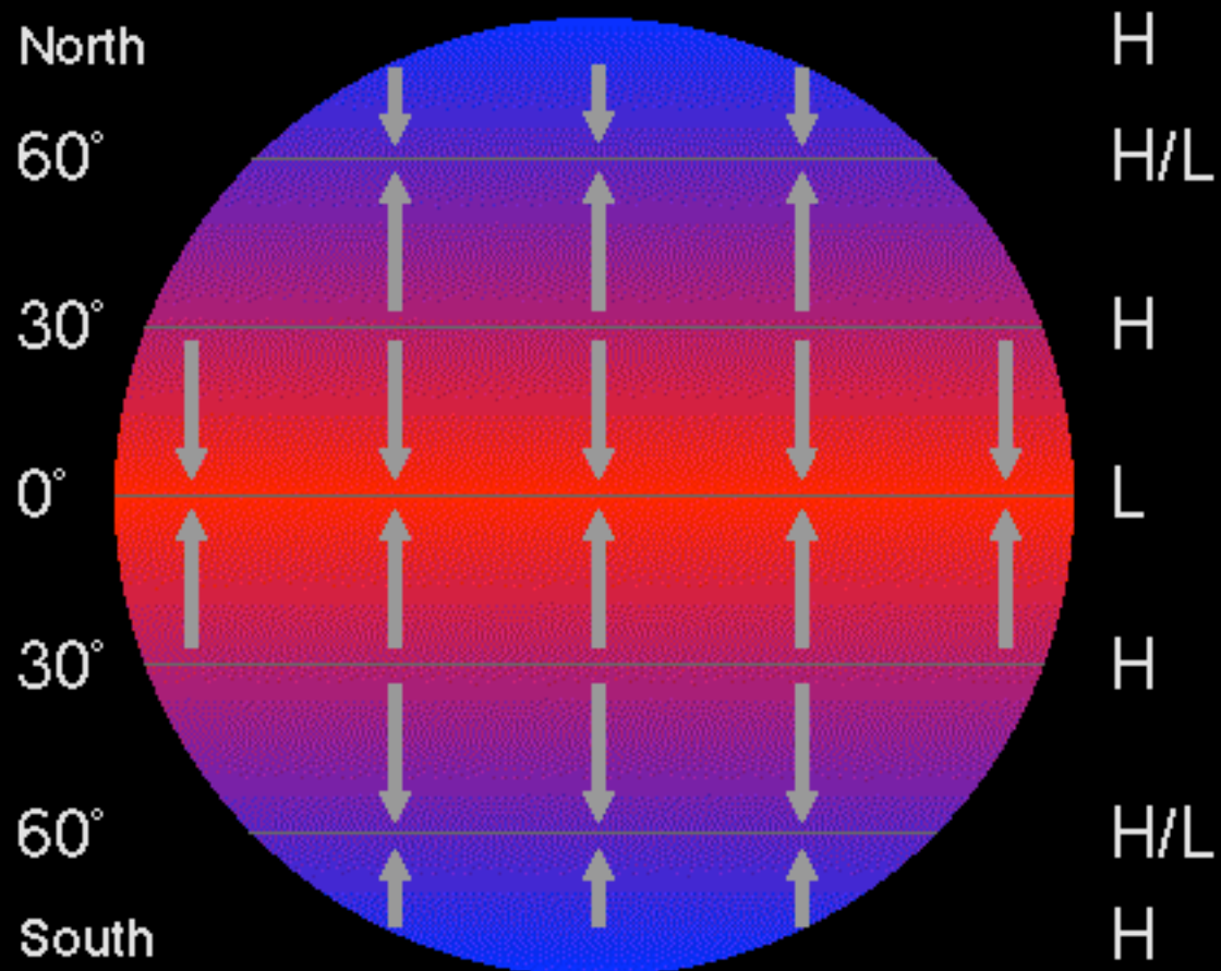
Basic Surface Windfield
