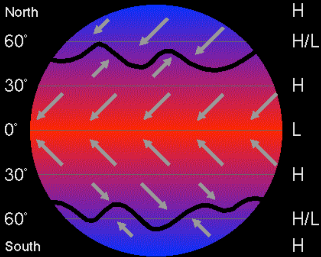
Coriolis Surface Windfield w/Polar Front Zone
